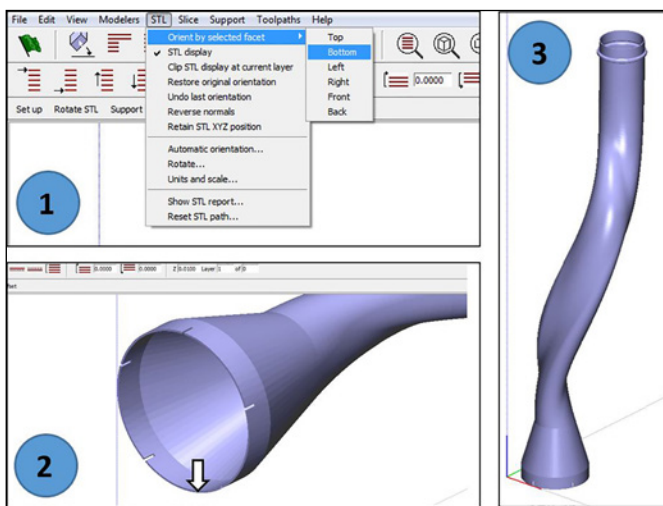
Figure 12: In this example, selecting "bottom" (1), and then selecting the flat end of the duct (2) makes this face the bottom of the part in the build envelope (3).
