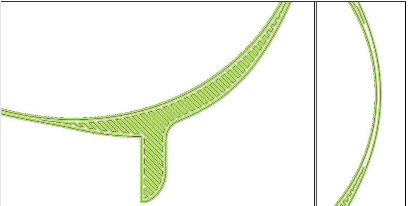
Figure 7: Thick parts with variation are filled by rasters (left) but thin, variable cross-sections cause voiding between the inner and outer contour (right).
