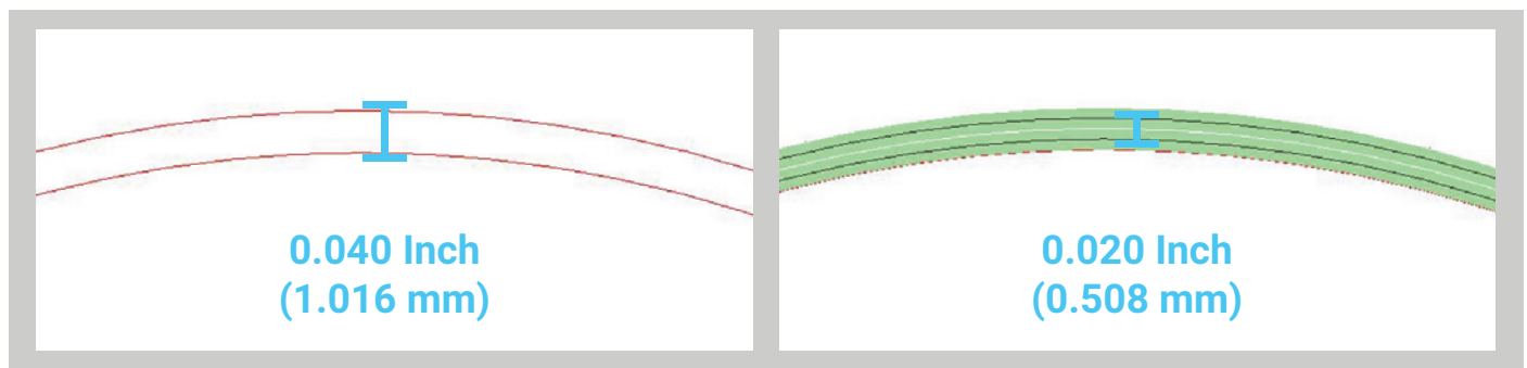
Figure 3: The minimum recommended wall thickness for FDM ducting (left) in order to properly fill the geometry with the standard toolpaths (right).
