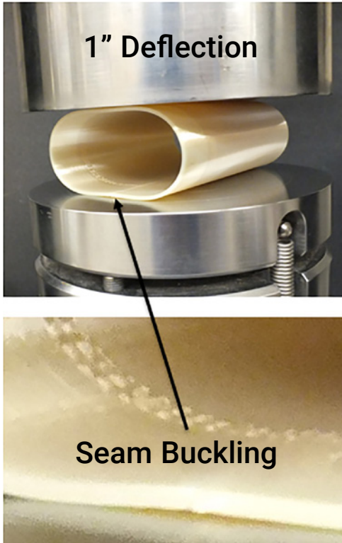
Figure 42: Deflection testing of four-contour ULTEM™ 9085 resin duct.
