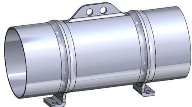
Figure 10: Additive manufacturing allows for integrated features and part consolidation.
