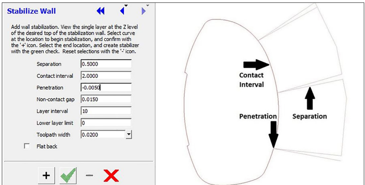
Figure 23: A stabilizer wall tailored to the specific part geometry.
