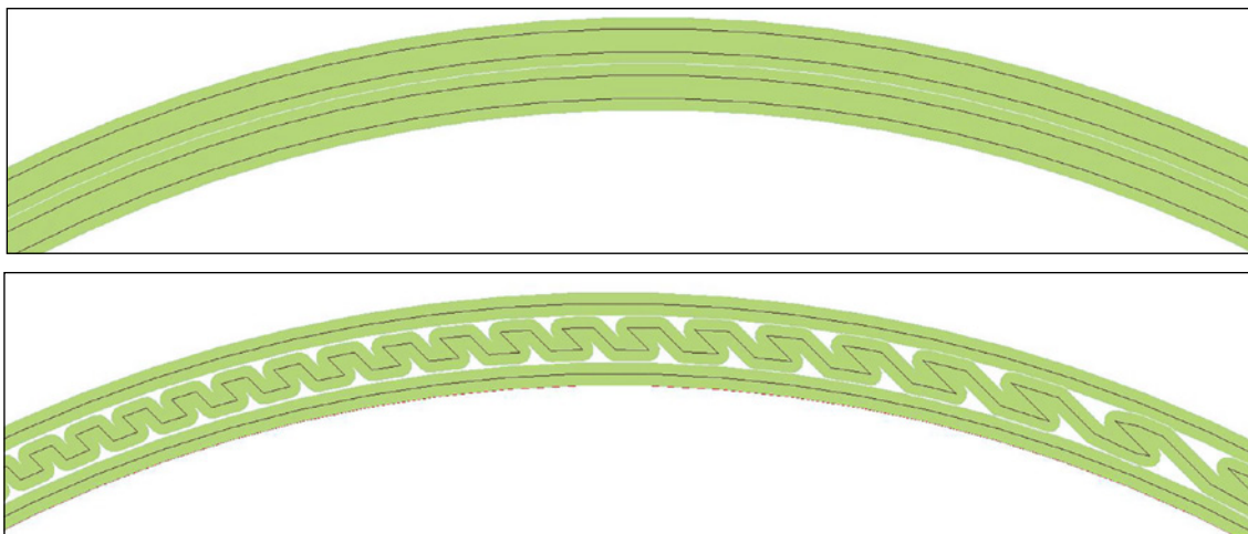
Figure 35: A duct consisting of four contours compared to a duct of two contours with a raster fill in between.
