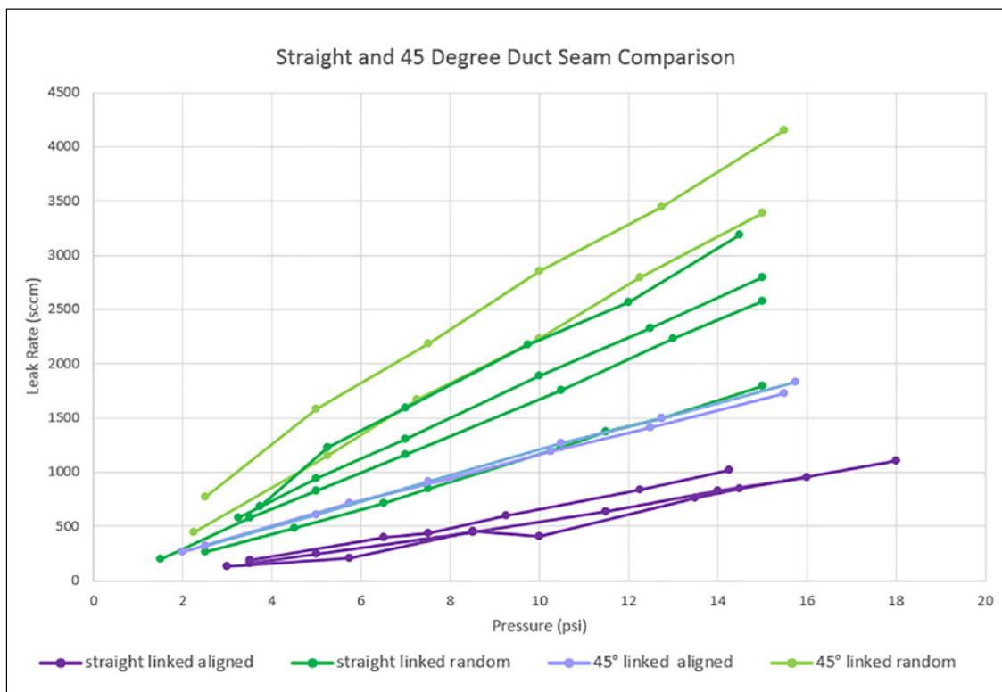
Figure 34: Leak rate comparison between straight and 45-degree ducts.
