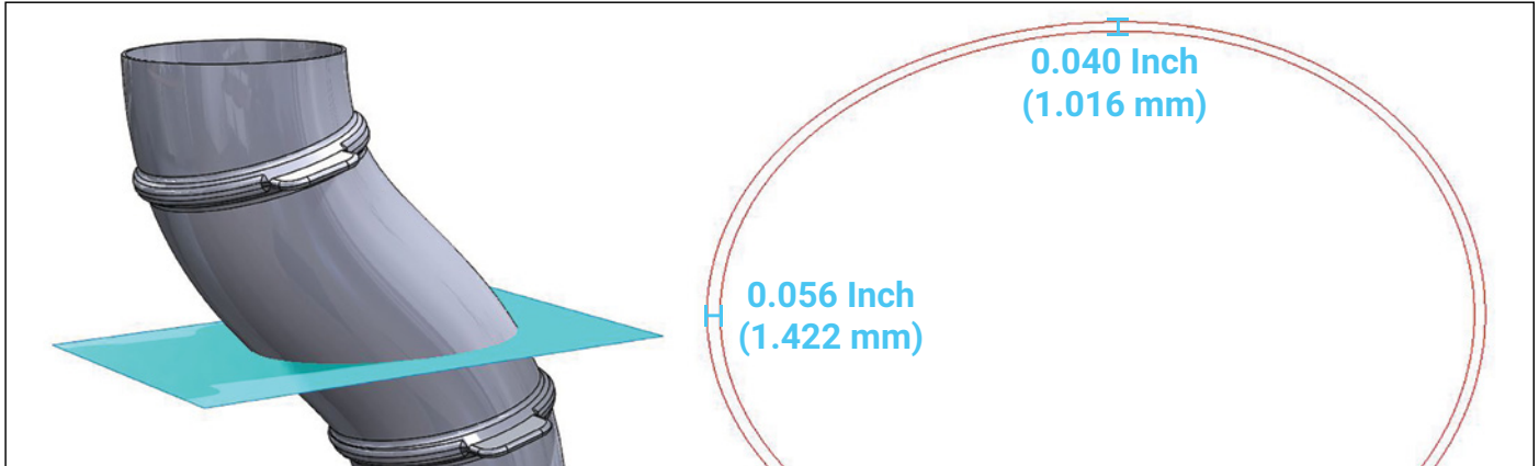
Figure 6: A duct with a constant 0.040 inch (1.016 mm) wall thickness yields a varying cross-sectional thickness (right) when sliced into two-dimensional curves in angled areas of the duct, as indicated by the blue plane (left).
