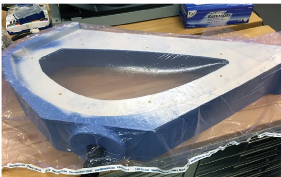
Figure 11. Test setup to evaluate the effectiveness of using spray paint to effectively seal the edges of the vacuum fixture.
