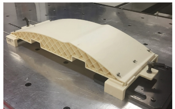
Figure 6. FDM machining fixture secured to the CNC platen.
